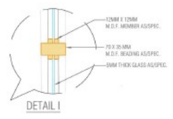
DETAIL H
