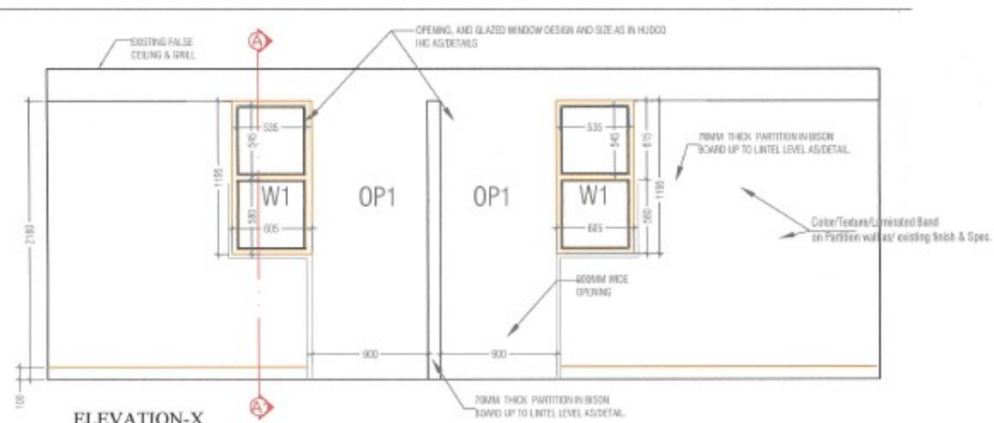
ELEVATION-X
